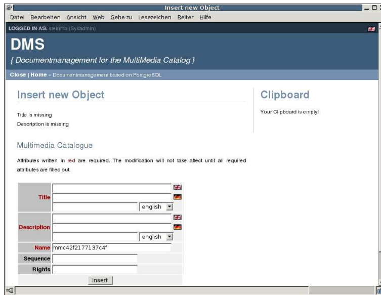
Figure 3: Adding the MULTIMEDIA CATALOGUE.
